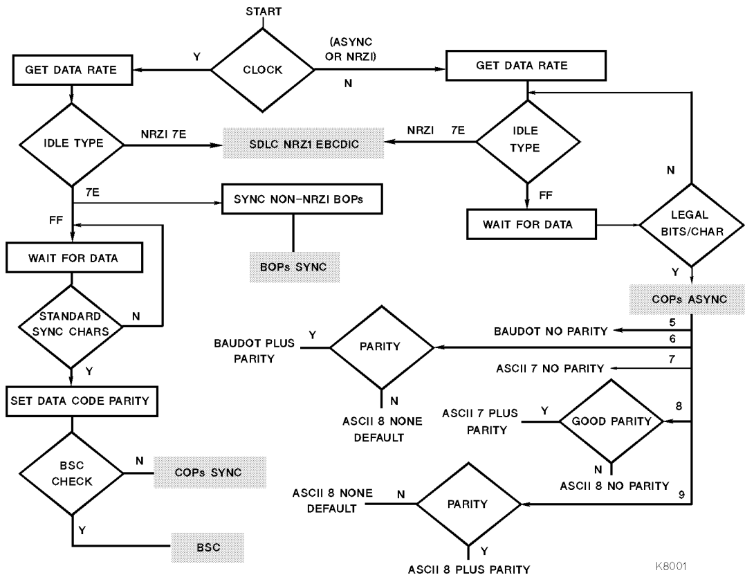
Figure 4-2: Auto Configure Algorithm
