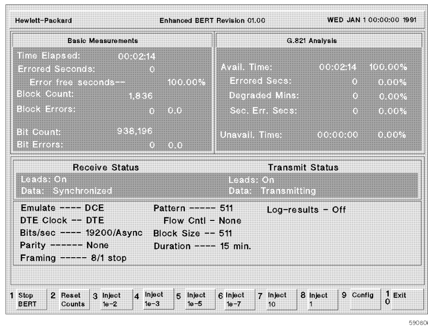
Figure 8-4: The BERT Measurement Window
