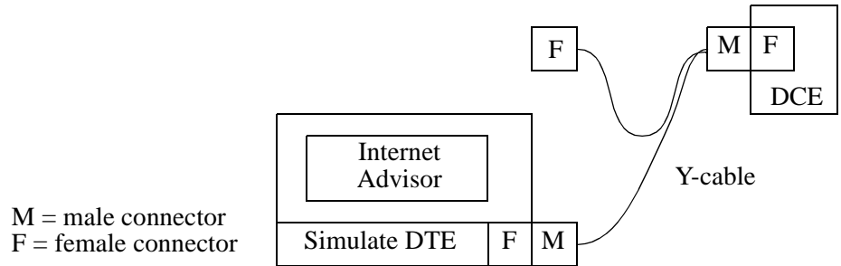
Figure 2-4: V-Series Active Connections to Test DCE and Link
